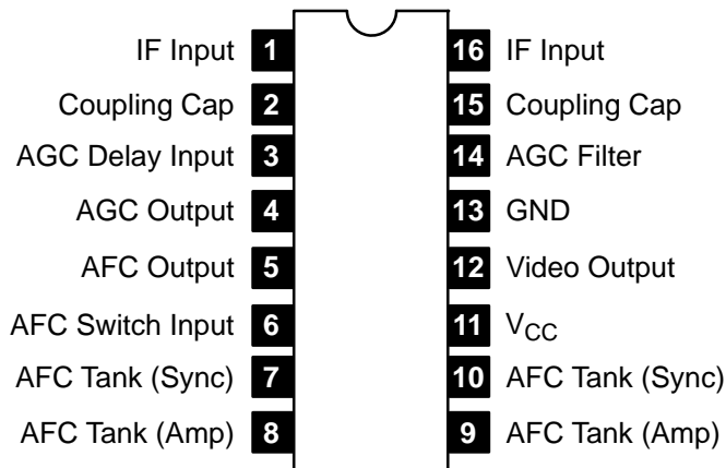
Pin Connection Diagram
